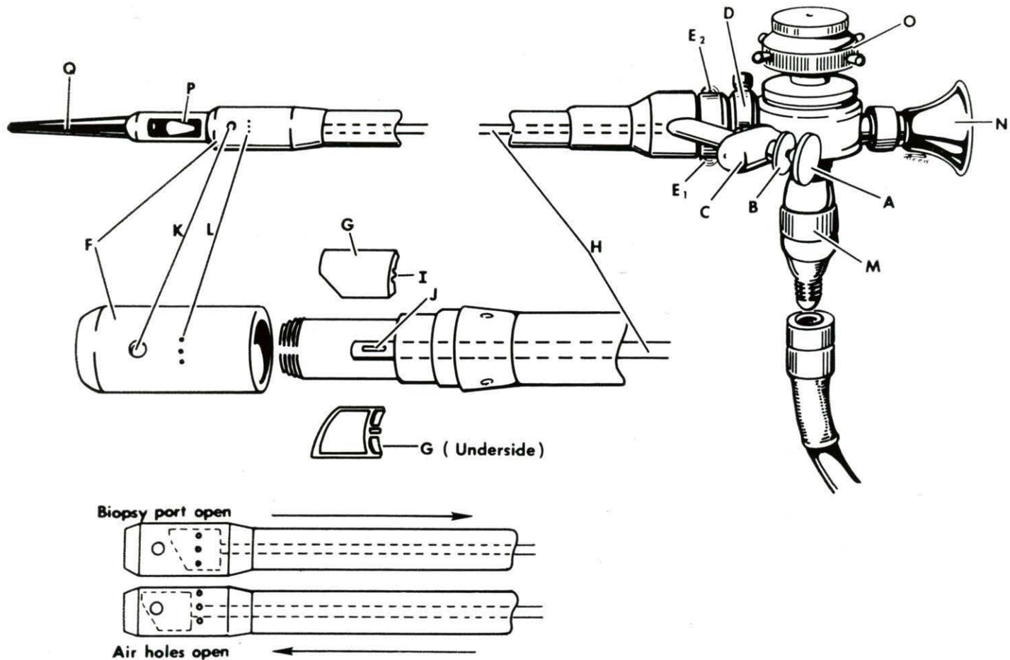
Fig. 21-5. Berry biopsy instrument, schematic drawing. A, Cutting plunger; B, flanged bushing; C, slotted bushing; D, locknut; E 1 inflation connector; E 2 , suction connector; F, cutting head; G, biopsy knife; H, cutting wire; I, knife key; J, cutting wire key slot; K, biopsy port; L, air holes. Eder-Palmer gastroscope parts also shown include: M, light switch; N, eyepiece; O, remote control handle; P, objective window; Q, tip.
